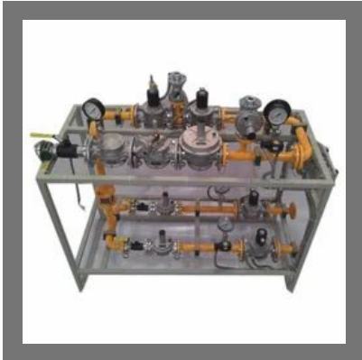
2 Zone Output And Individual Zone Gas Train
